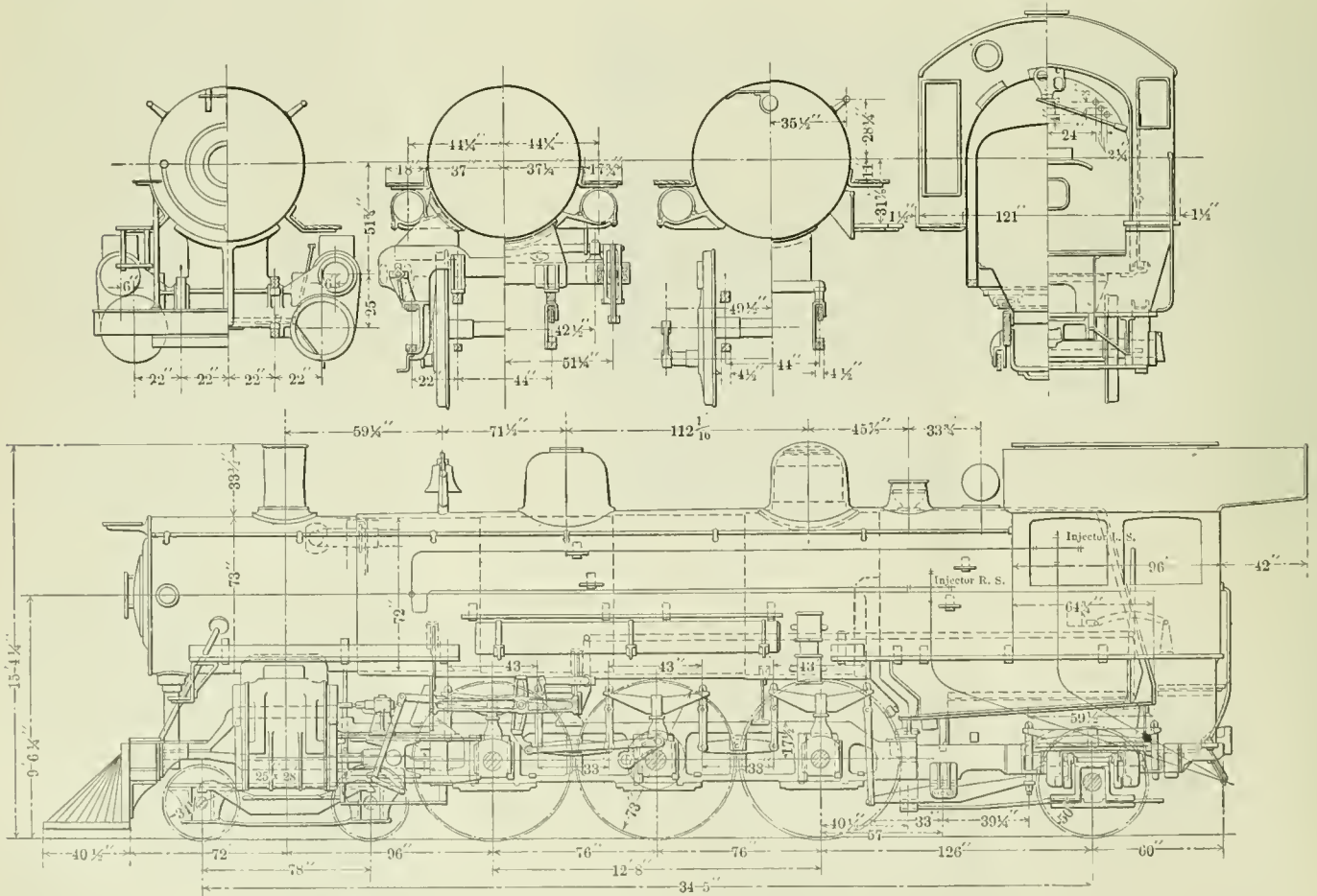
ELEVATIONS AND SECTIONS OF PACIFIC TYPE LOCOMOTIVE—A. T. & S. F. RY.
